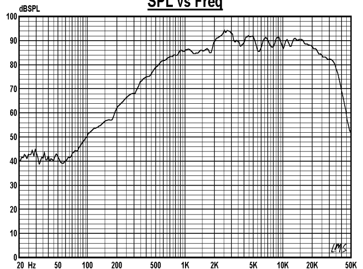
SPL vs Freq
