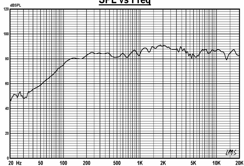
SPL vs Freq
